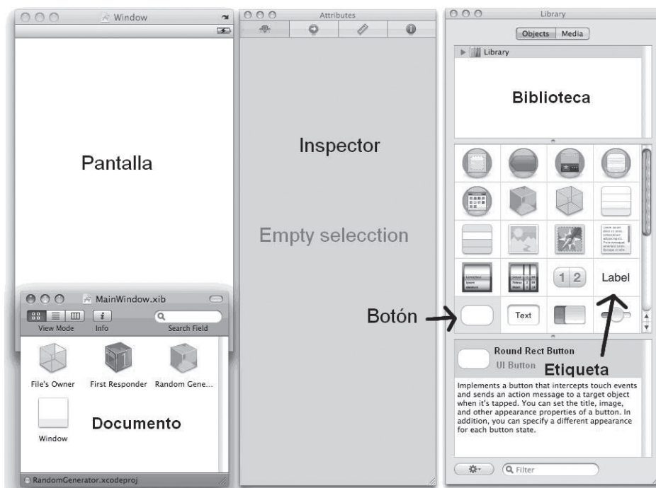
Figura 1.18. Herramienta Builder
