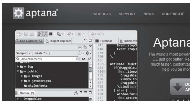
Figura 1.15. Aptana Studio
