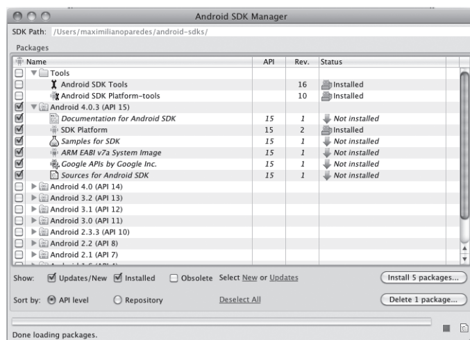
Figura 1.14. AVD Manager
